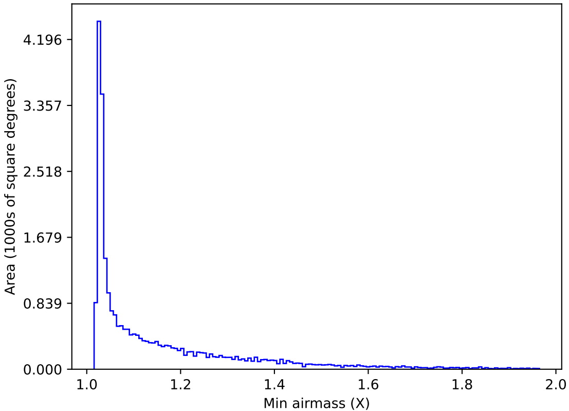
too_elab_r8_d3_ugrizy_v3.4_10yrs All sky z band: Min airmass
