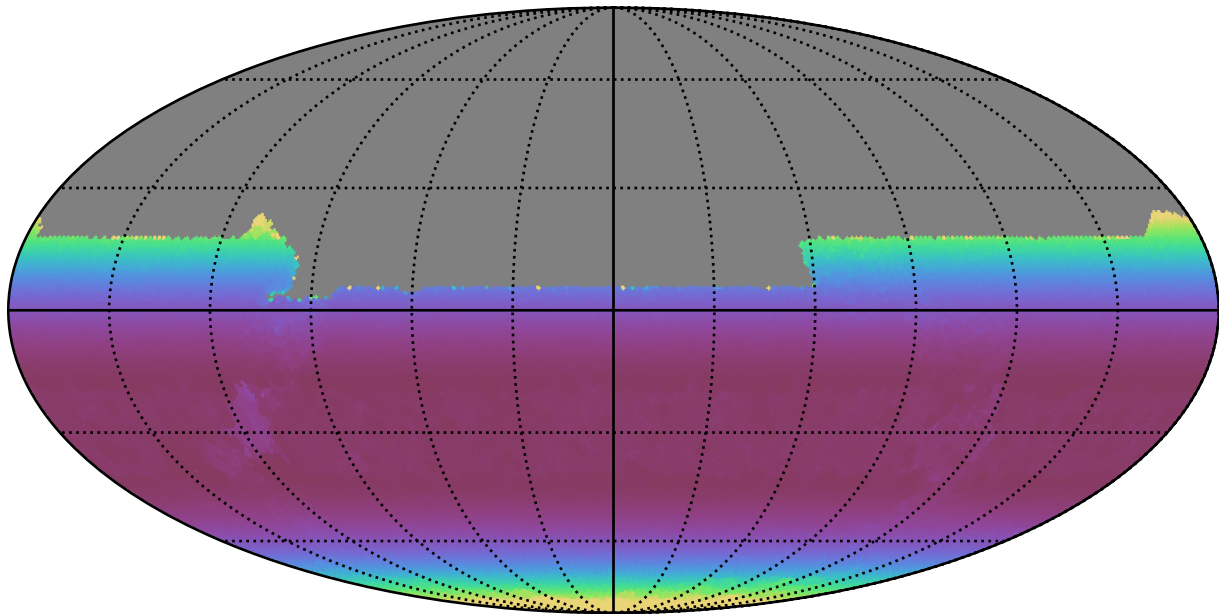
too_elab_r8_d3_ugrizy_v3.4_10yrs All sky y band: Min airmass
