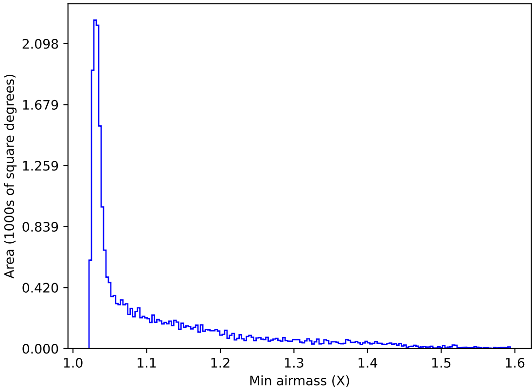
too_elab_r8_d3_ugrizy_v3.4_10yrs All sky y band: Min airmass
