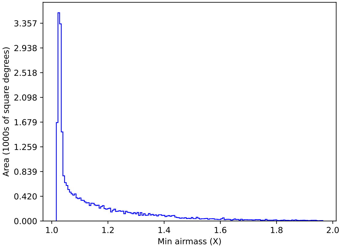
too_elab_r8_d3_ugrizy_v3.4_10yrs All sky r band: Min airmass
