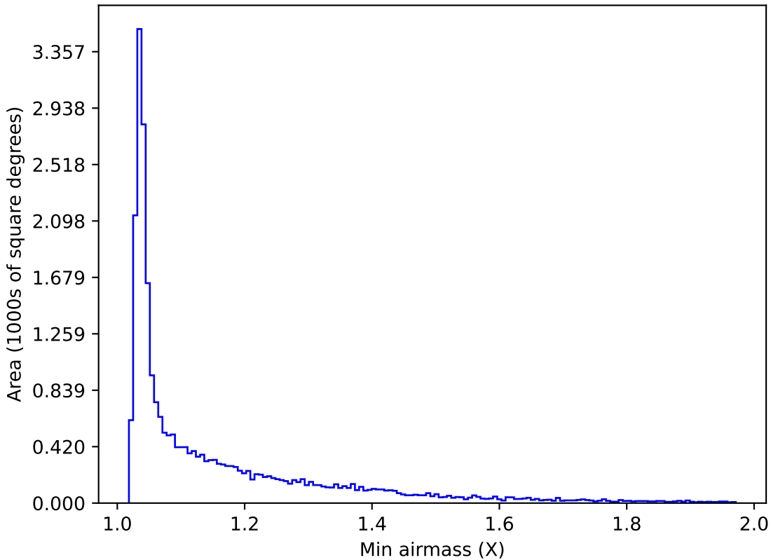
too_elab_r8_d3_ugrizy_v3.4_10yrs All sky g band: Min airmass
