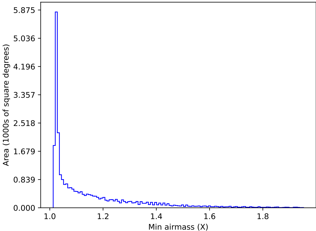
too_elab_r8_d3_ugrizy_v3.4_10yrs All sky all bands: Min airmass
