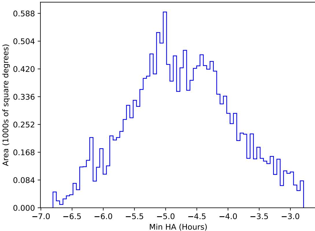
too_elab_r8_d3_ugrizy_v3.4_10yrs WFD all bands: Min HA
