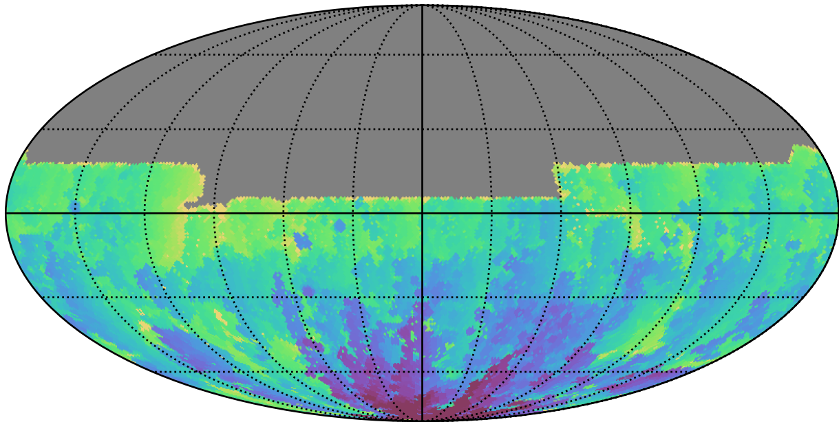
too_elab_r8_d3_ugrizy_v3.4_10yrs All sky u band: Min HA
