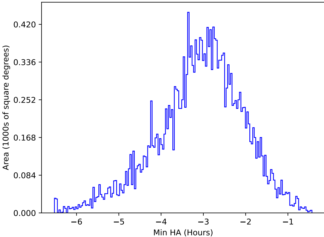
too_elab_r8_d3_ugrizy_v3.4_10yrs All sky u band: Min HA
