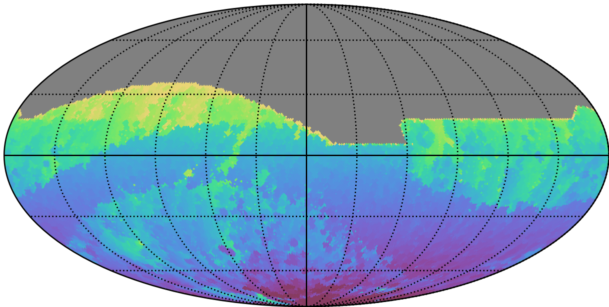
too_elab_r8_d3_ugrizy_v3.4_10yrs All sky r band: Min HA
