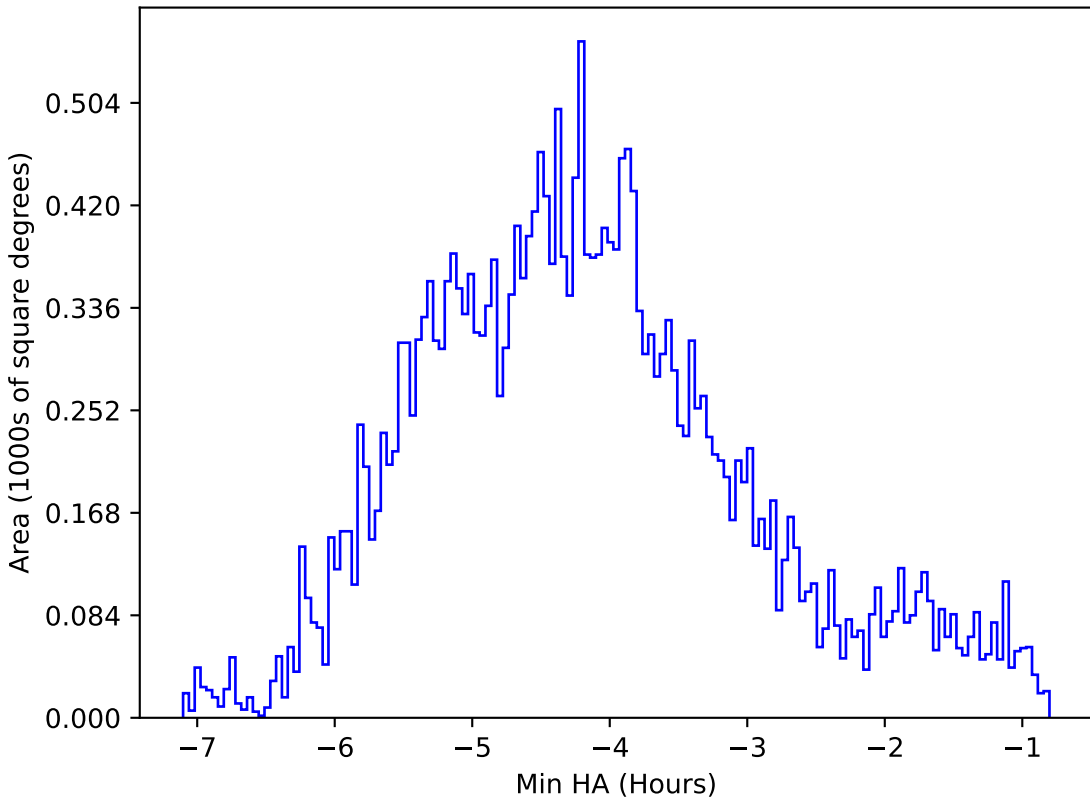
too_elab_r8_d3_ugrizy_v3.4_10yrs All sky r band: Min HA
