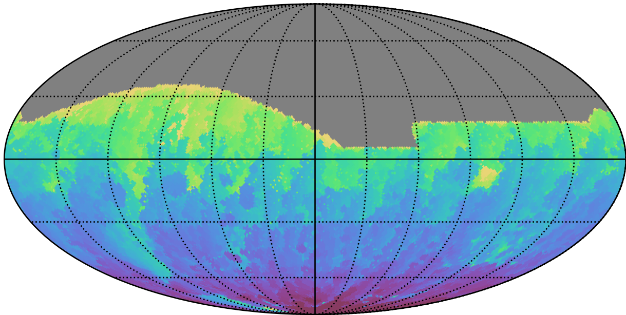
too_elab_r8_d3_ugrizy_v3.4_10yrs All sky g band: Min HA
