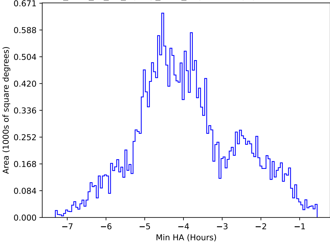
too_elab_r8_d3_ugrizy_v3.4_10yrs All sky g band: Min HA
