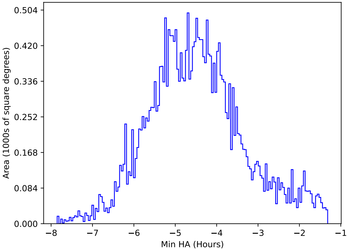
too_elab_r8_d3_ugrizy_v3.4_10yrs All sky all bands: Min HA
