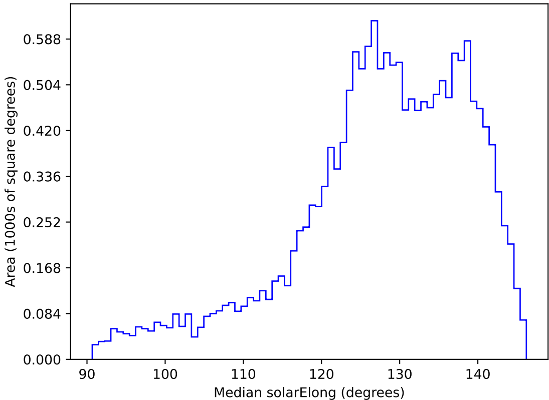
too_elab_r8_d3_ugrizy_v3.4_10yrs WFD z band: Median solarElong
