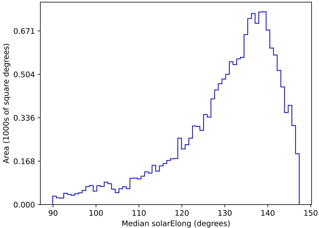
too_elab_r8_d3_ugrizy_v3.4_10yrs WFD r band: Median solarElong
