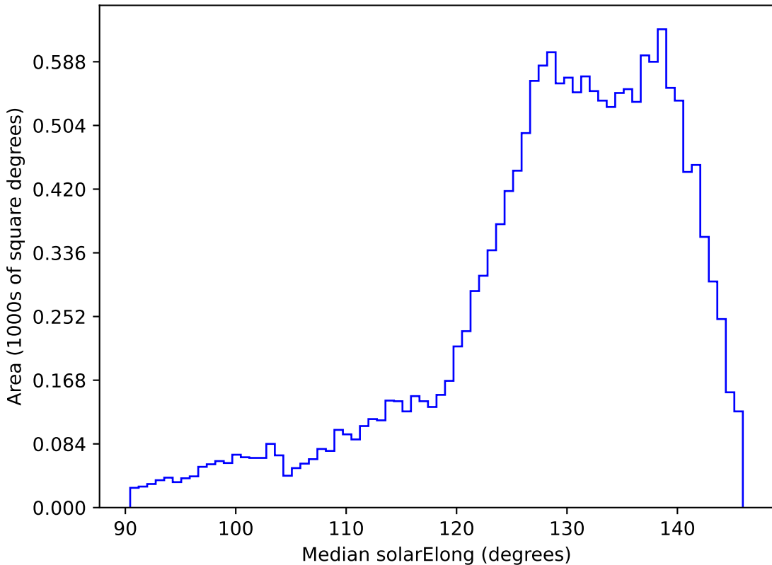
too_elab_r8_d3_ugrizy_v3.4_10yrs WFD i band: Median solarElong
