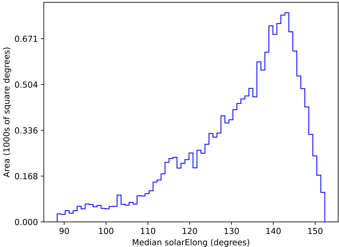
too_elab_r8_d3_ugrizy_v3.4_10yrs WFD g band: Median solarElong
