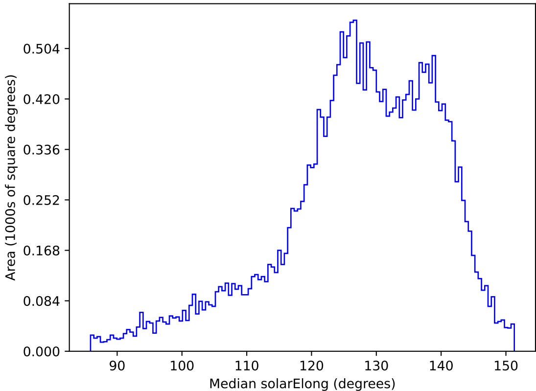
too_elab_r8_d3_ugrizy_v3.4_10yrs All sky z band: Median solarElong
