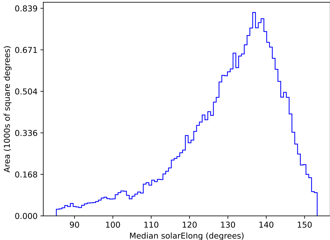
too_elab_r8_d3_ugrizy_v3.4_10yrs All sky r band: Median solarElong
