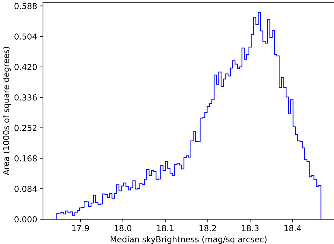
too_elab_r8_d3_ugrizy_v3.4_10yrs Yr 1 y band: Median skyBrightness
