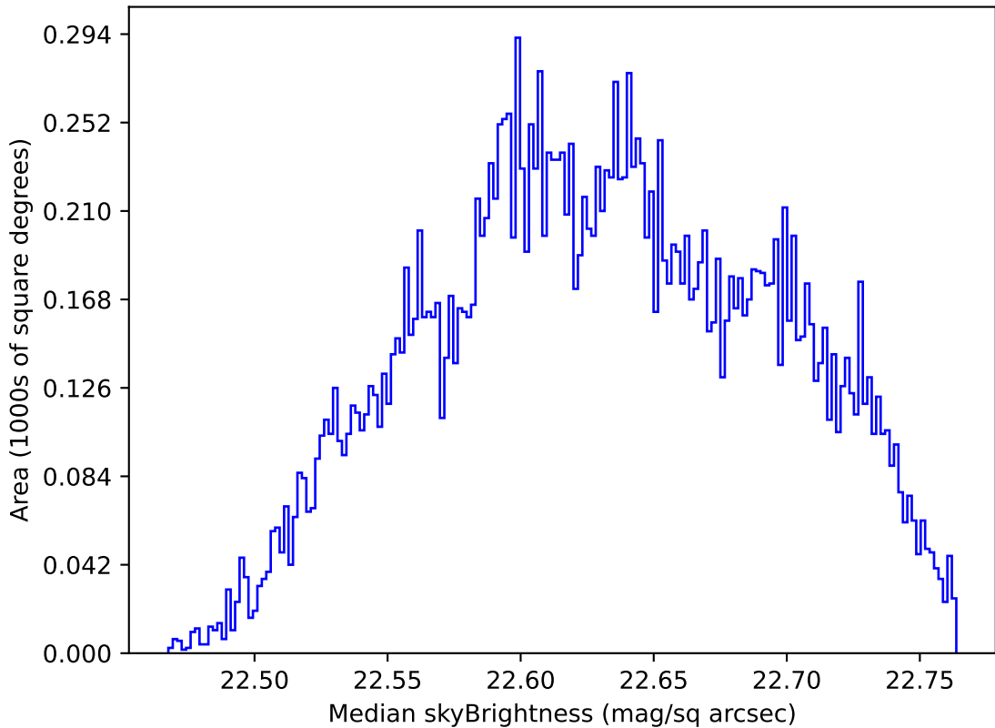
too_elab_r8_d3_ugrizy_v3.4_10yrs Yr 1 u band: Median skyBrightness
