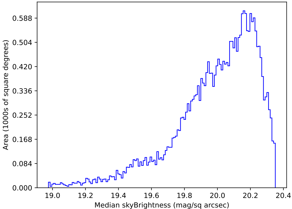
too_elab_r8_d3_ugrizy_v3.4_10yrs Yr 1 i band: Median skyBrightness
