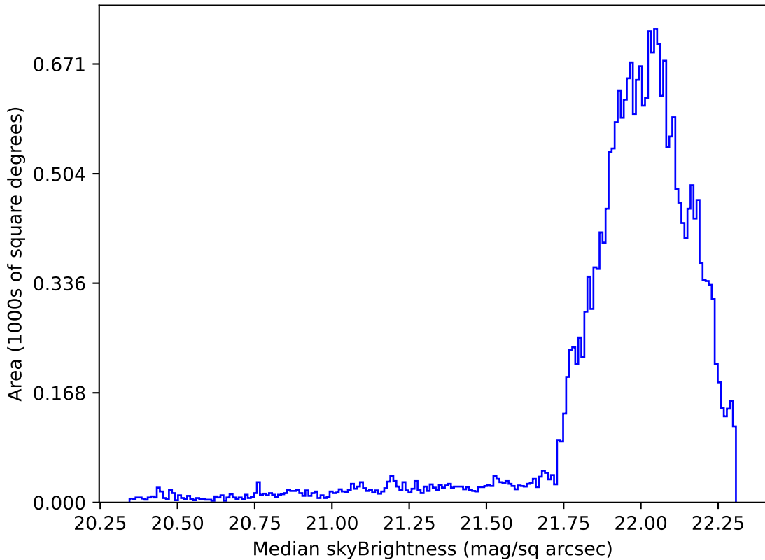
too_elab_r8_d3_ugrizy_v3.4_10yrs Yr 1 g band: Median skyBrightness
