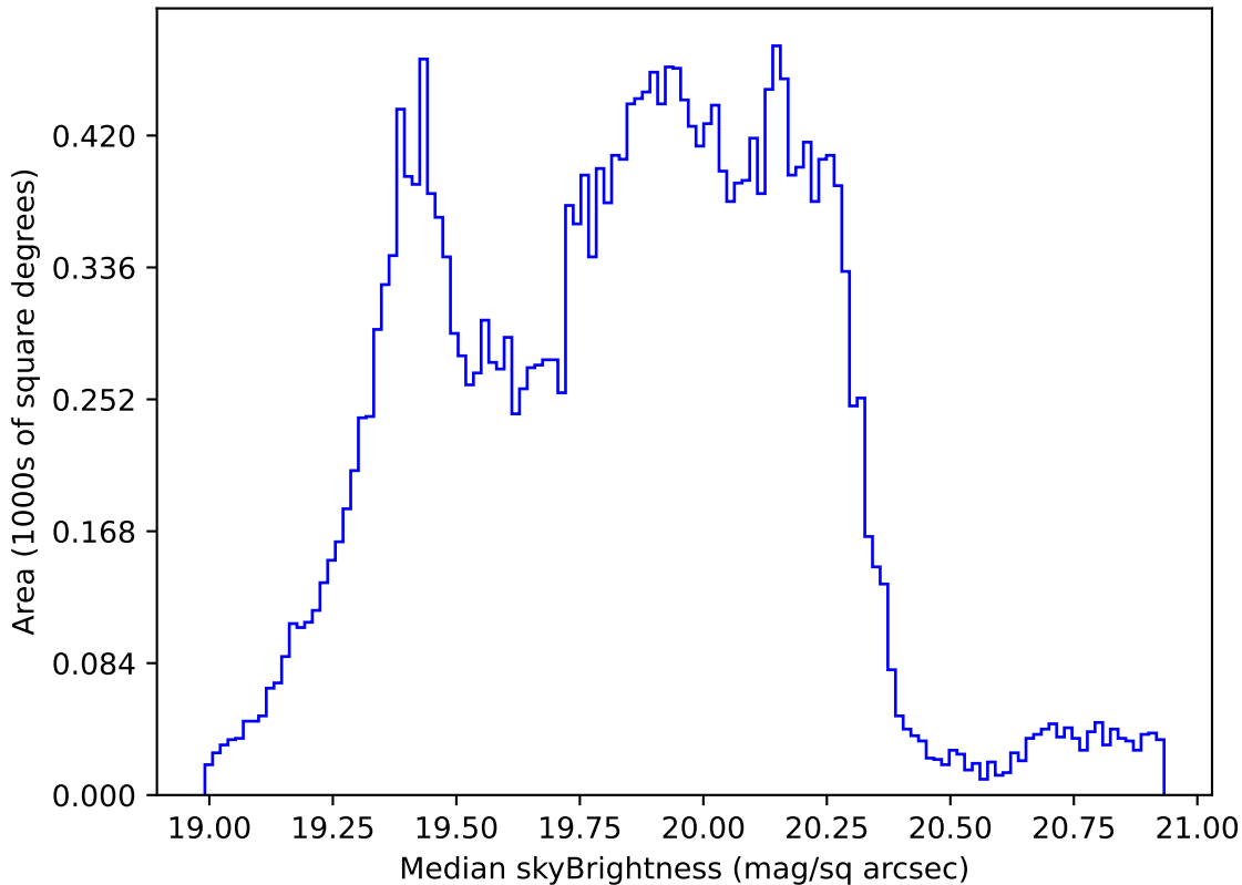
too_elab_r8_d3_ugrizy_v3.4_10yrs Yr 1 all bands: Median skyBrightness
