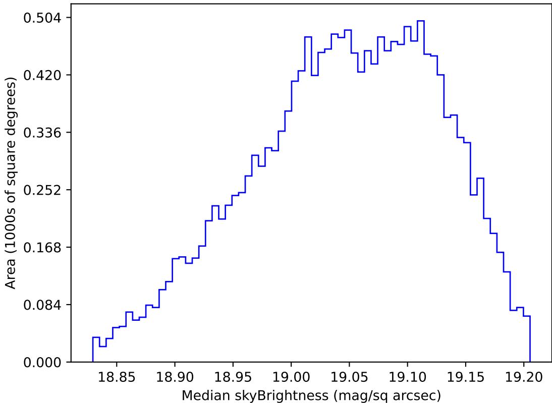
too_elab_r8_d3_ugrizy_v3.4_10yrs WFD z band: Median skyBrightness
