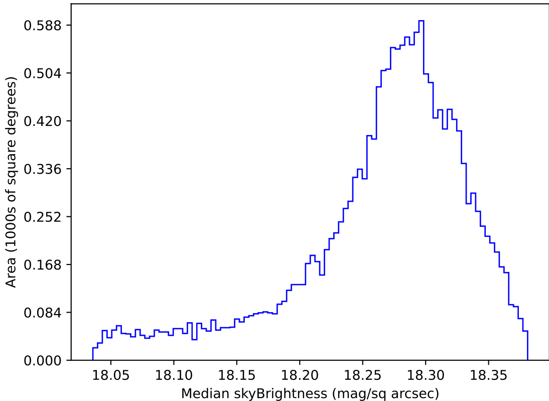
too_elab_r8_d3_ugrizy_v3.4_10yrs WFD y band: Median skyBrightness
