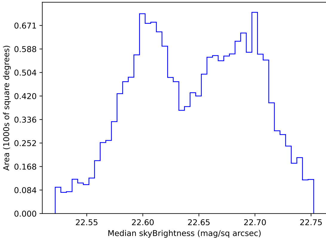
too_elab_r8_d3_ugrizy_v3.4_10yrs WFD u band: Median skyBrightness
