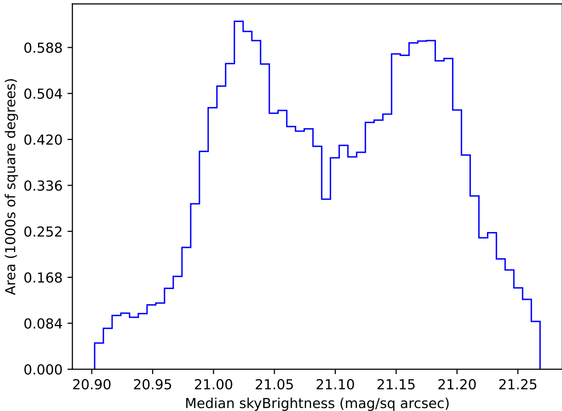
too_elab_r8_d3_ugrizy_v3.4_10yrs WFD r band: Median skyBrightness
