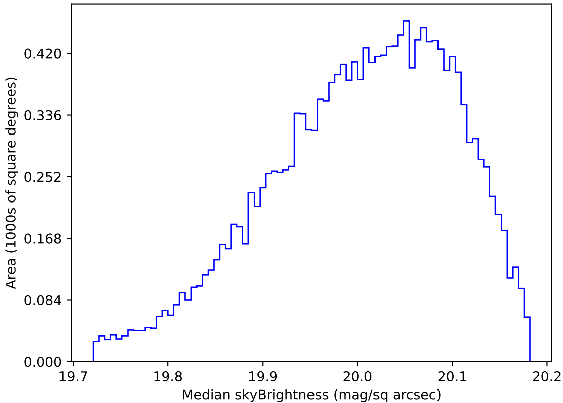
too_elab_r8_d3_ugrizy_v3.4_10yrs WFD i band: Median skyBrightness
