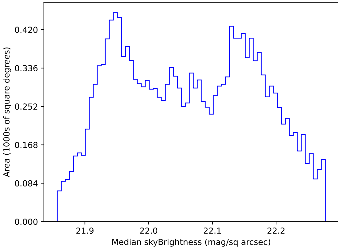
too_elab_r8_d3_ugrizy_v3.4_10yrs WFD g band: Median skyBrightness
