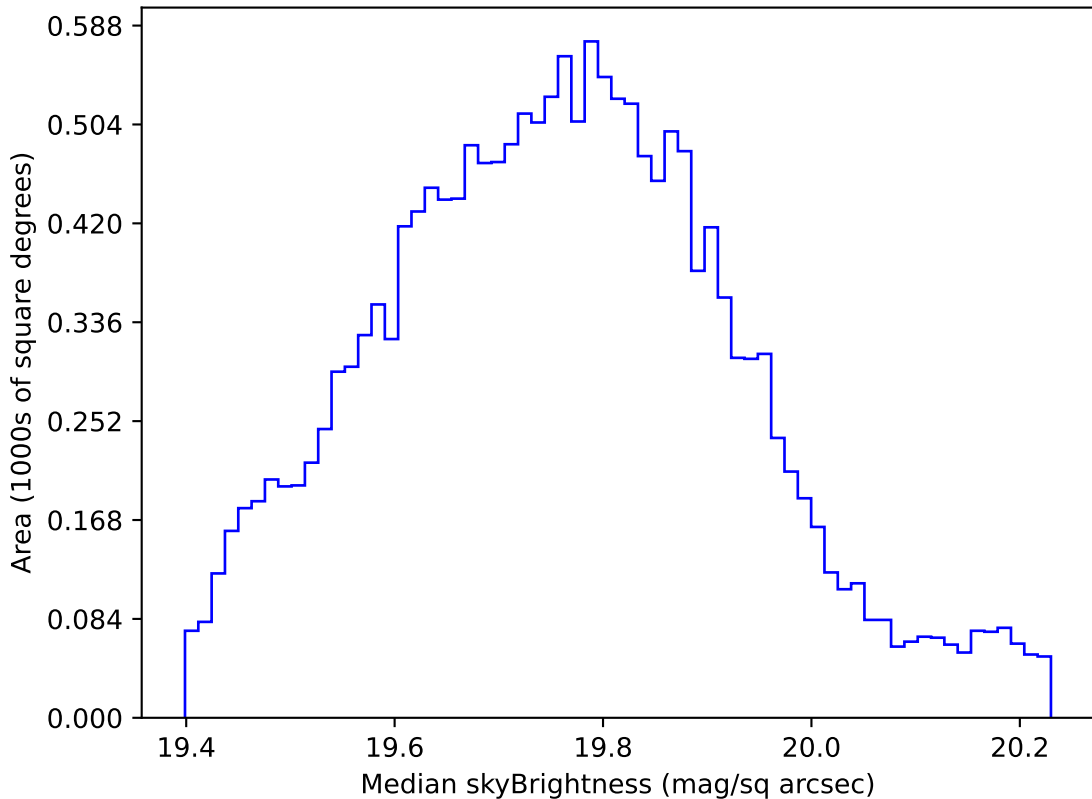
too_elab_r8_d3_ugrizy_v3.4_10yrs WFD all bands: Median skyBrightness
