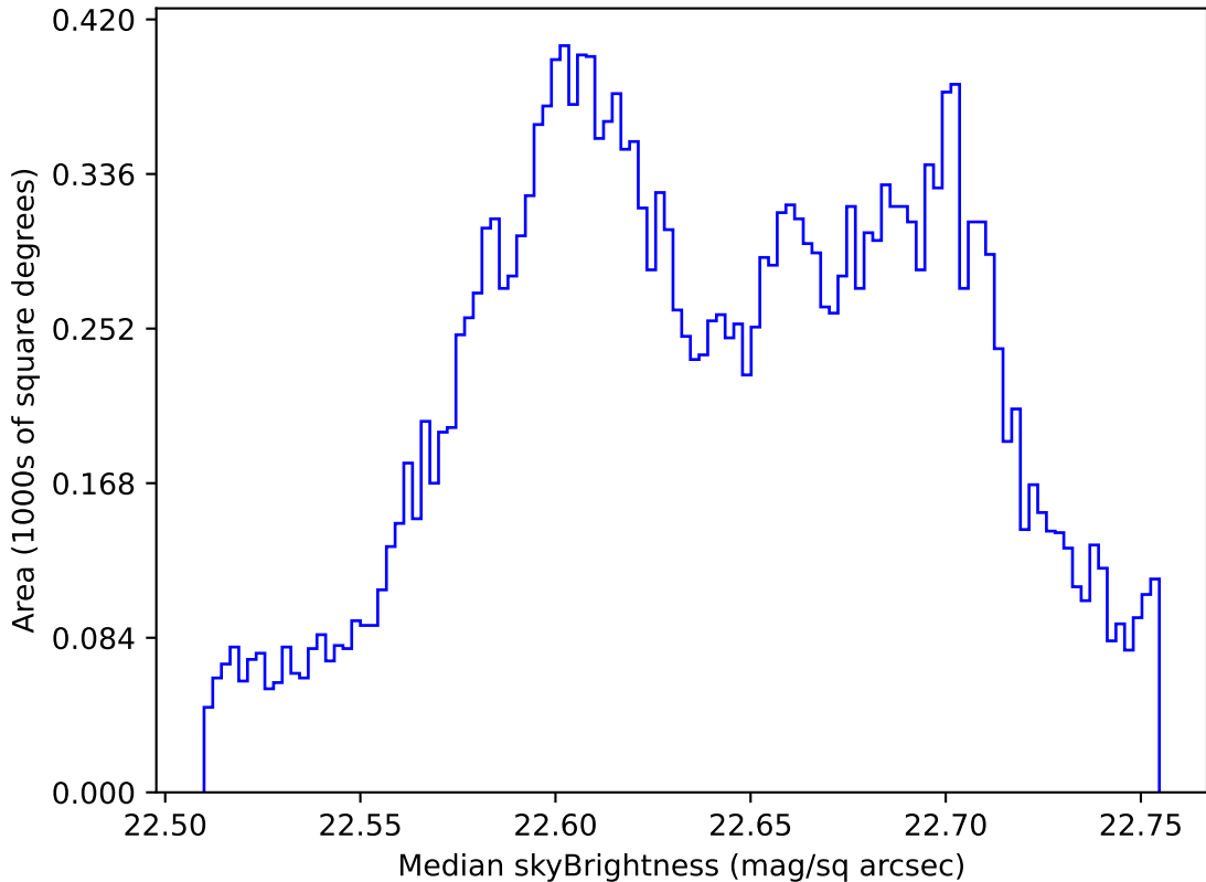
too_elab_r8_d3_ugrizy_v3.4_10yrs All sky u band: Median skyBrightness
