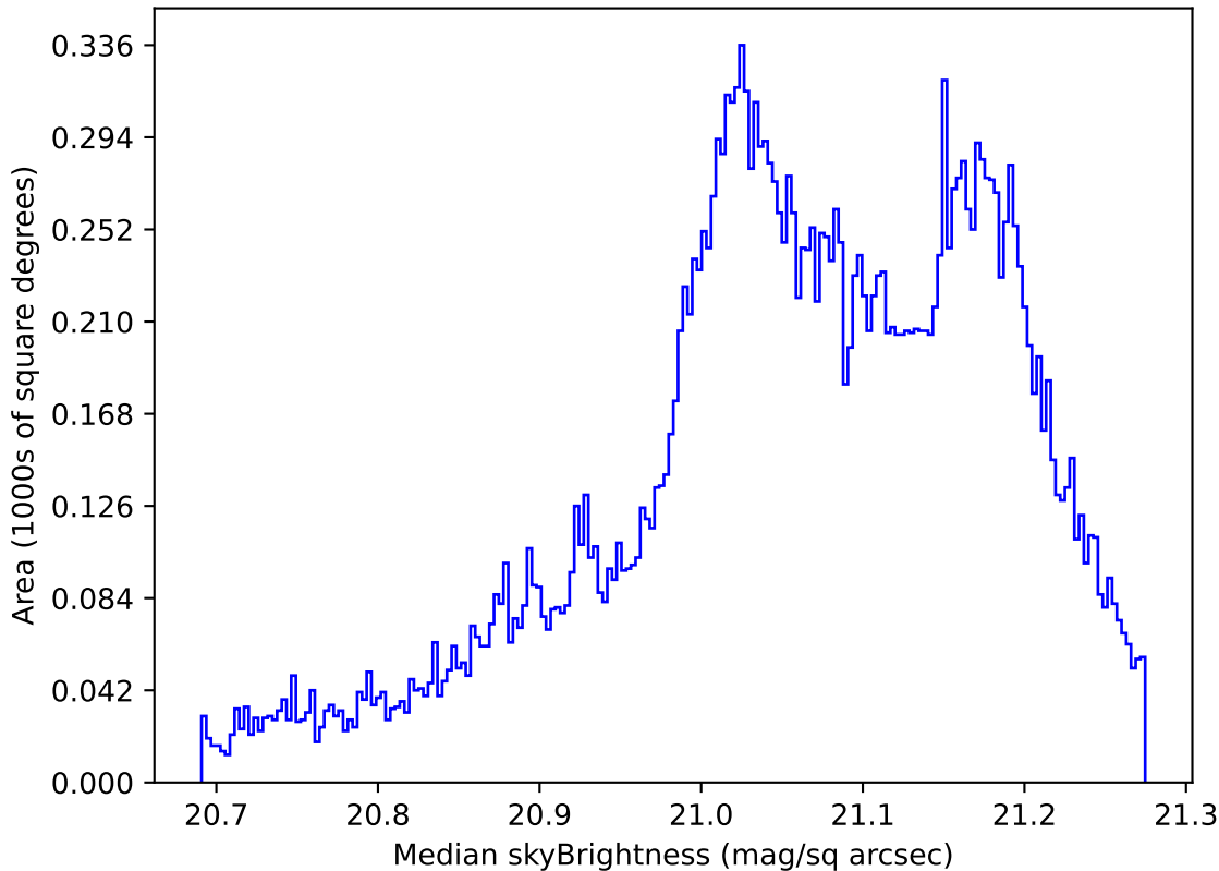
too_elab_r8_d3_ugrizy_v3.4_10yrs All sky r band: Median skyBrightness
