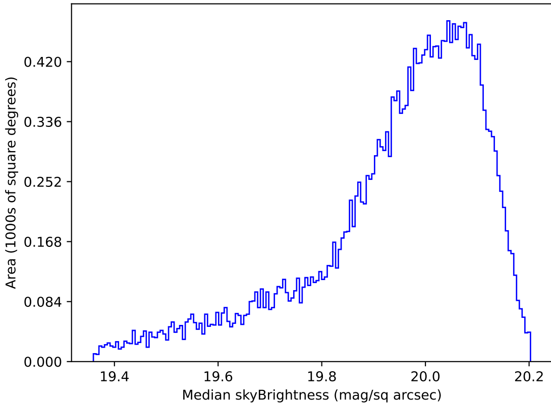
too_elab_r8_d3_ugrizy_v3.4_10yrs All sky i band: Median skyBrightness
