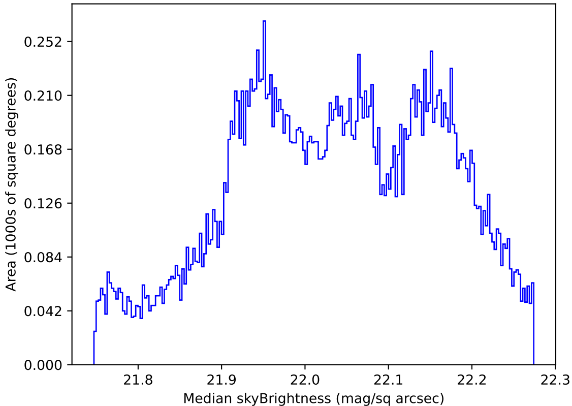
too_elab_r8_d3_ugrizy_v3.4_10yrs All sky g band: Median skyBrightness
