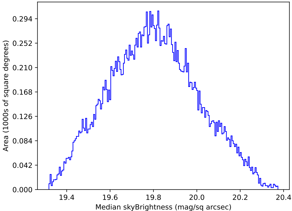
too_elab_r8_d3_ugrizy_v3.4_10yrs All sky all bands: Median skyBrightness
