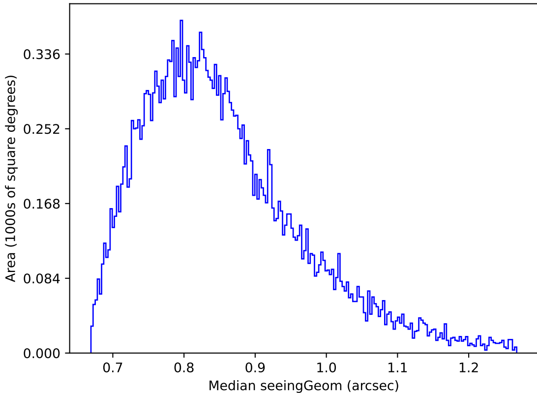
too_elab_r8_d3_ugrizy_v3.4_10yrs Yr 1 z band: Median seeingGeom
