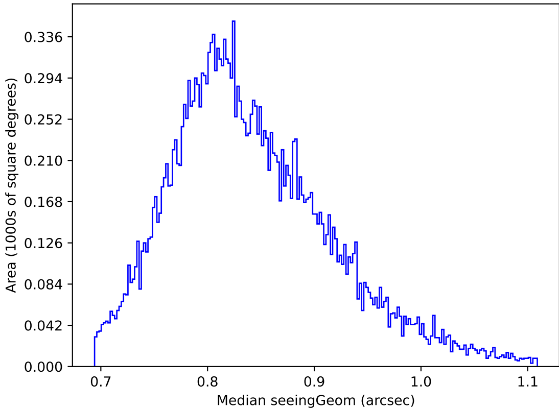
too_elab_r8_d3_ugrizy_v3.4_10yrs Yr 1 y band: Median seeingGeom
