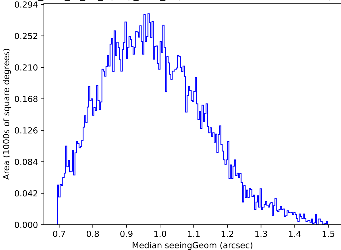
too_elab_r8_d3_ugrizy_v3.4_10yrs Yr 1 u band: Median seeingGeom
