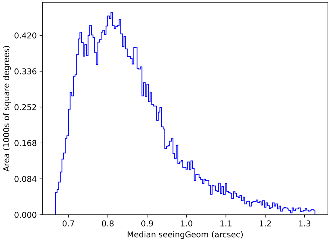
too_elab_r8_d3_ugrizy_v3.4_10yrs Yr 1 r band: Median seeingGeom
