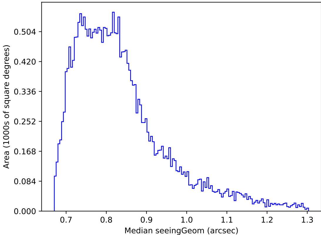
too_elab_r8_d3_ugrizy_v3.4_10yrs Yr 1 i band: Median seeingGeom
