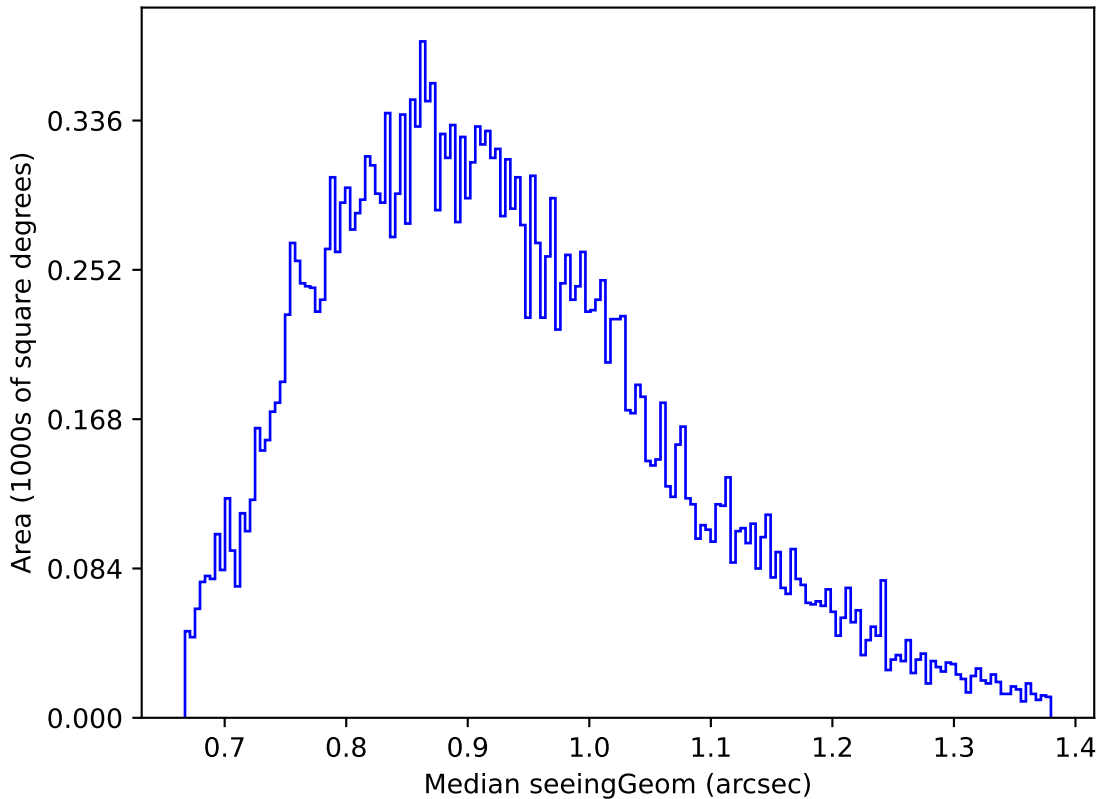
too_elab_r8_d3_ugrizy_v3.4_10yrs Yr 1 g band: Median seeingGeom
