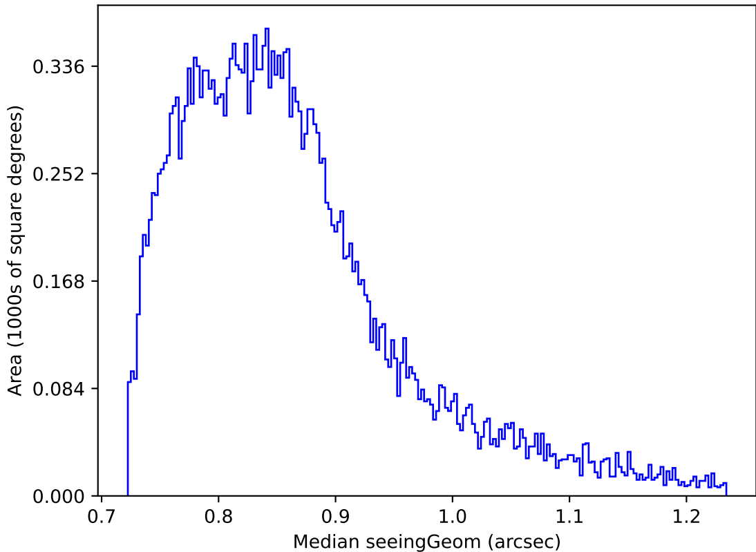
too_elab_r8_d3_ugrizy_v3.4_10yrs Yr 1 all bands: Median seeingGeom
