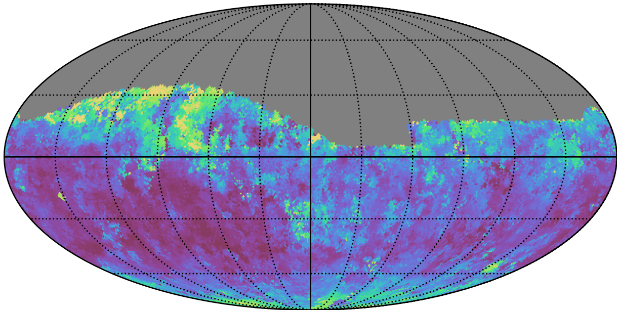
too_elab_r8_d3_ugrizy_v3.4_10yrs Yr 1 z band: Median seeingEff
