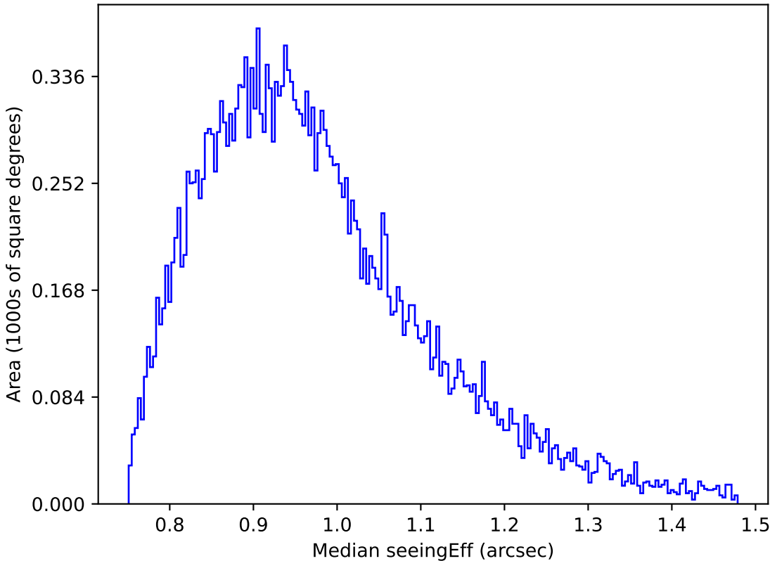
too_elab_r8_d3_ugrizy_v3.4_10yrs Yr 1 z band: Median seeingEff
