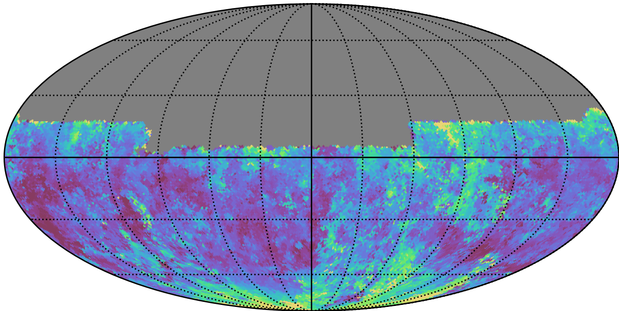
too_elab_r8_d3_ugrizy_v3.4_10yrs Yr 1 y band: Median seeingEff
