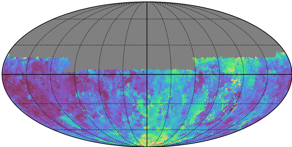
too_elab_r8_d3_ugrizy_v3.4_10yrs Yr 1 u band: Median seeingEff
