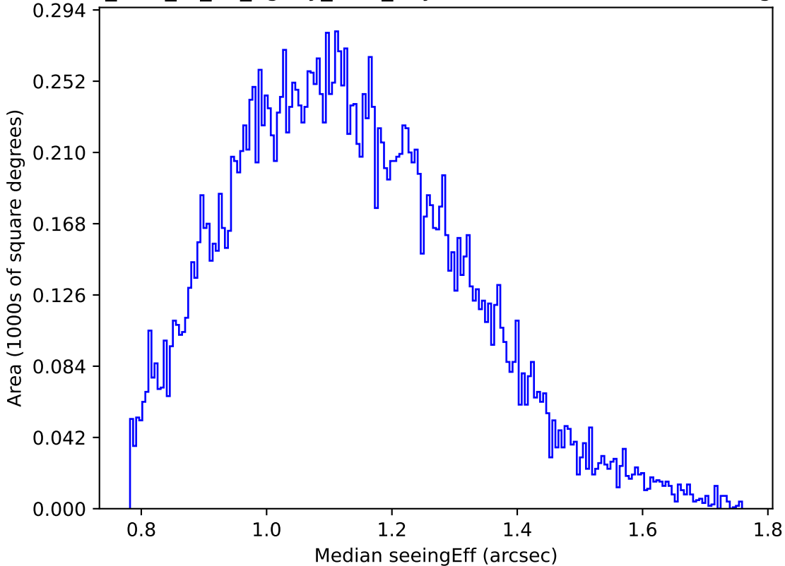
too_elab_r8_d3_ugrizy_v3.4_10yrs Yr 1 u band: Median seeingEff
