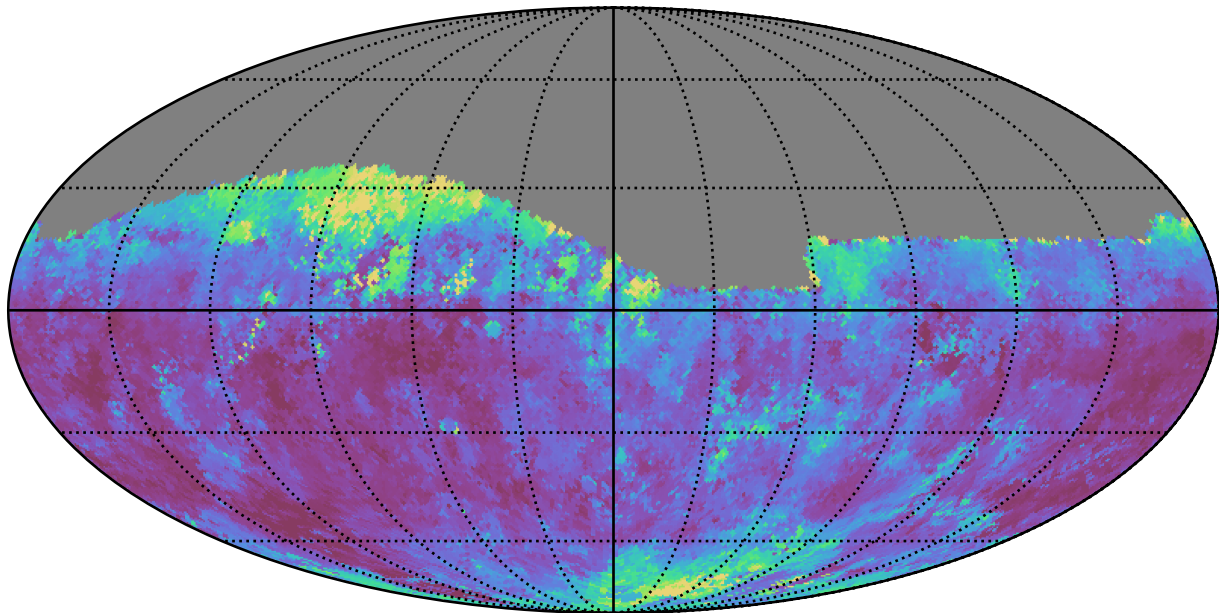
too_elab_r8_d3_ugrizy_v3.4_10yrs Yr 1 r band: Median seeingEff
